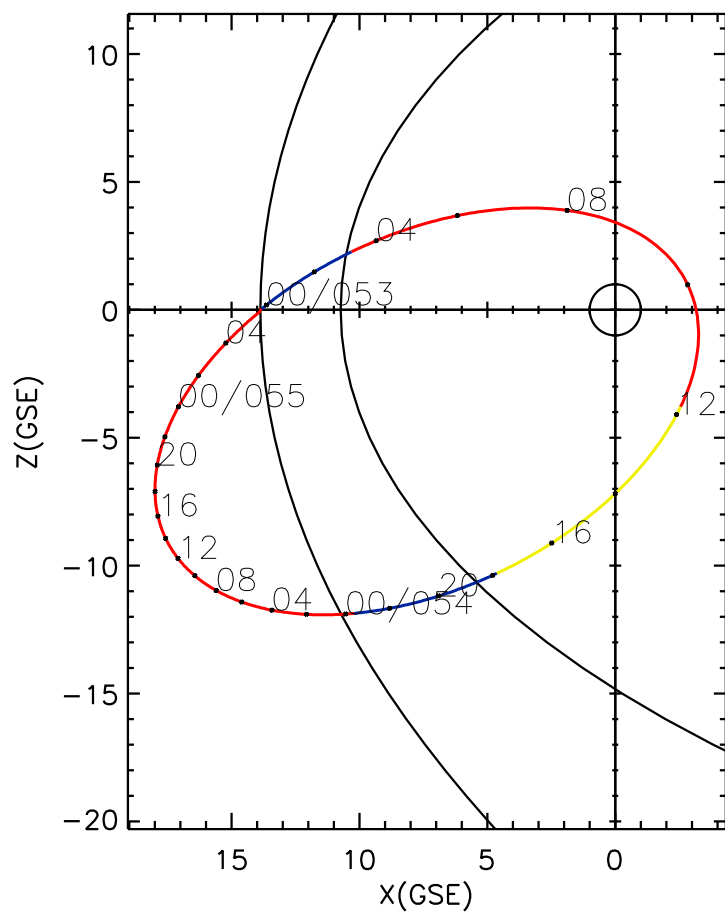
CLUSTER 2 orbit 2014 052 (02/21) 23:41 UT to 2014 055 (02/24) 05:56 UT
