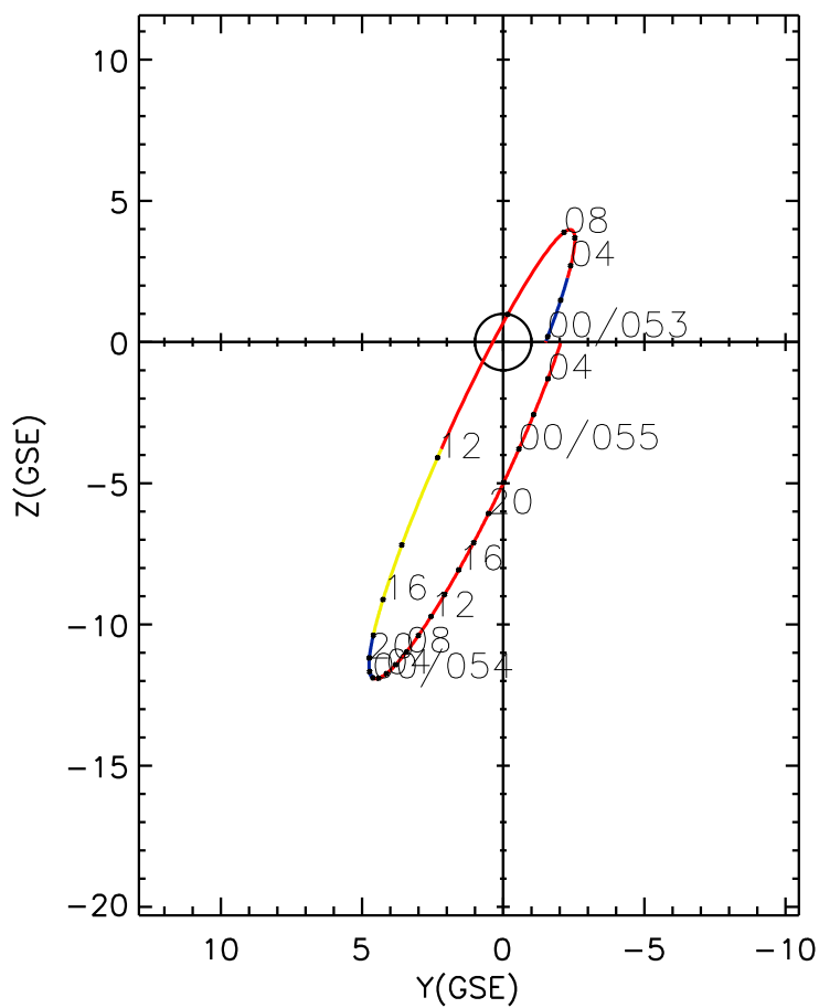
CLUSTER 2 orbit 2014 052 (02/21) 23:41 UT to 2014 055 (02/24) 05:56 UT
