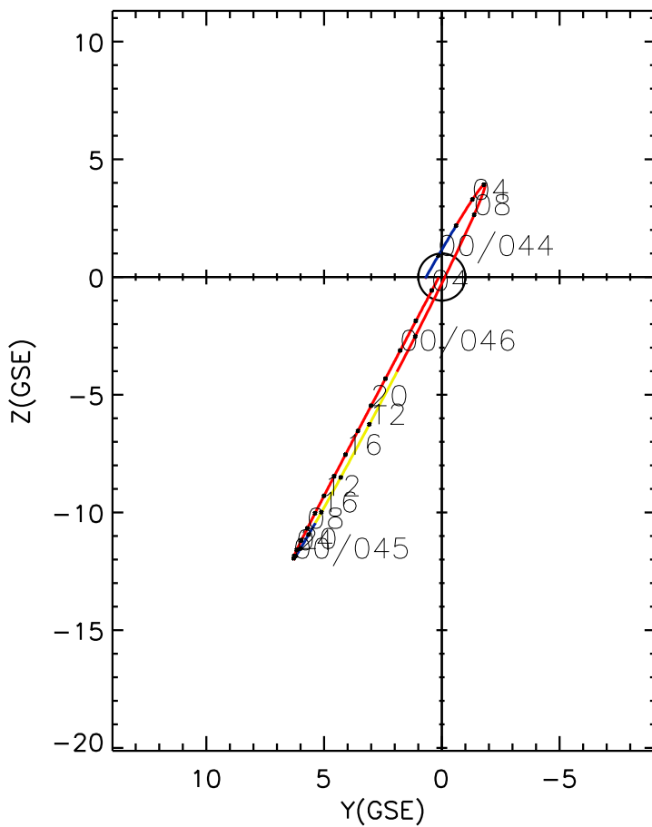
CLUSTER 2 orbit 2014 043 (02/12) 22:31 UT to 2014 046 (02/15) 04:51 UT
