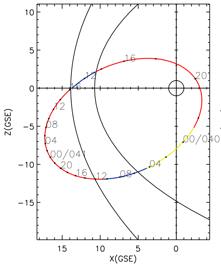
CLUSTER 2 orbit 2014 039 (02/08) 10:01 UT to 2014 041 (02/10) 16:16 UT
