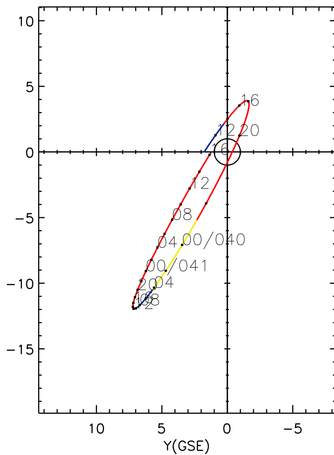
CLUSTER 2 orbit 2014 039 (02/08) 10:01 UT to 2014 041 (02/10) 16:16 UT
