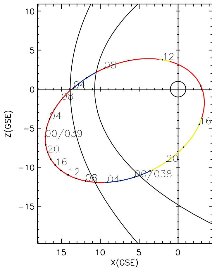
CLUSTER 2 orbit 2014 037 (02/06) 03:41 UT to 2014 039 (02/08) 10:01 UT
