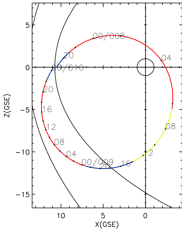
CLUSTER 2 orbit 2014 007 (01/07) 18:16 UT to 2014 010 (01/10) 00:31 UT
