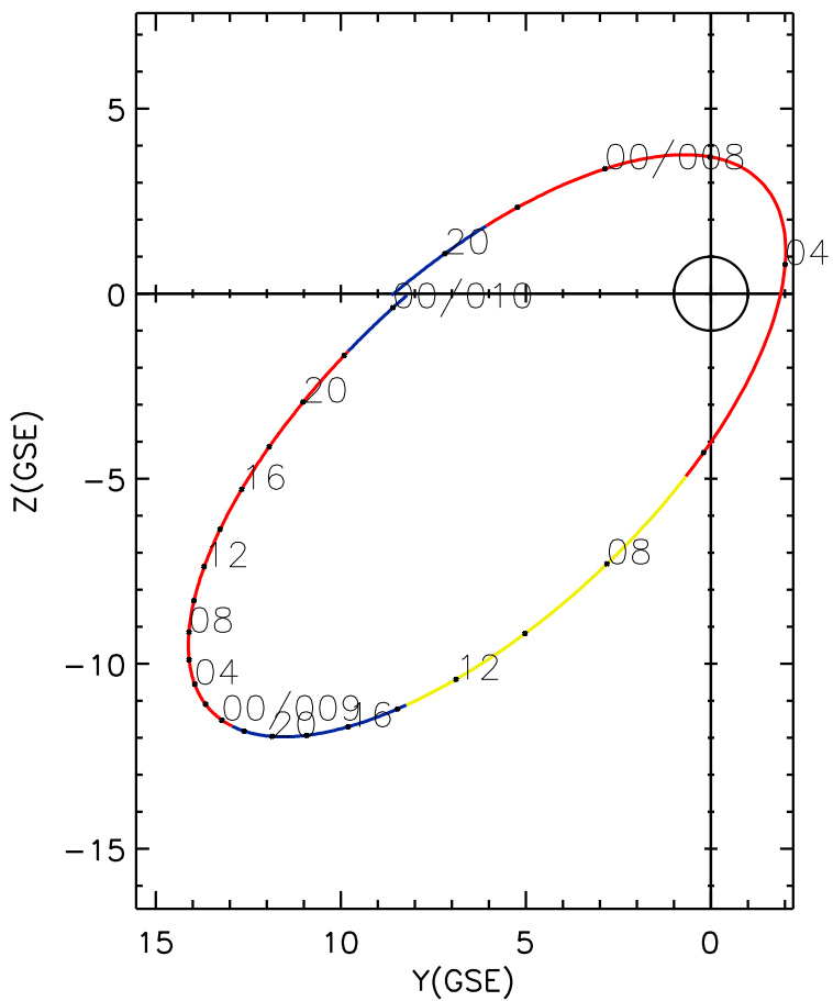
CLUSTER 2 orbit 2014 007 (01/07) 18:16 UT to 2014 010 (01/10) 00:31 UT
