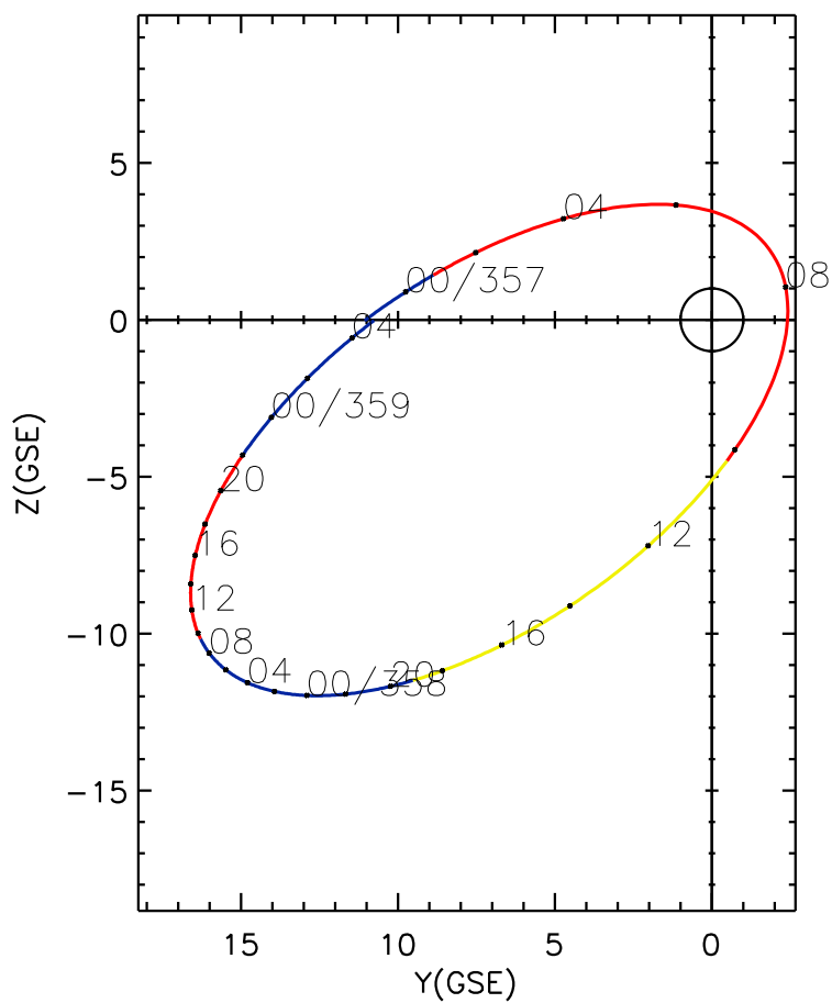
CLUSTER 2 orbit 2013 356 (12/22) 22:36 UT to 2013 359 (12/25) 04:51 UT
