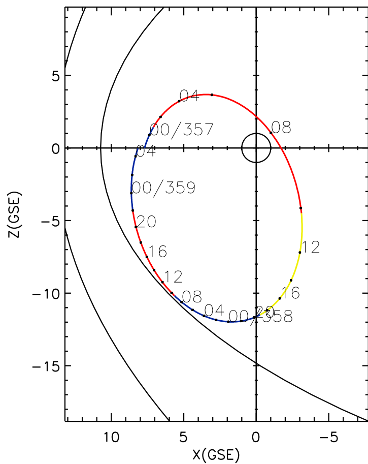
CLUSTER 2 orbit 2013 356 (12/22) 22:36 UT to 2013 359 (12/25) 04:51 UT
