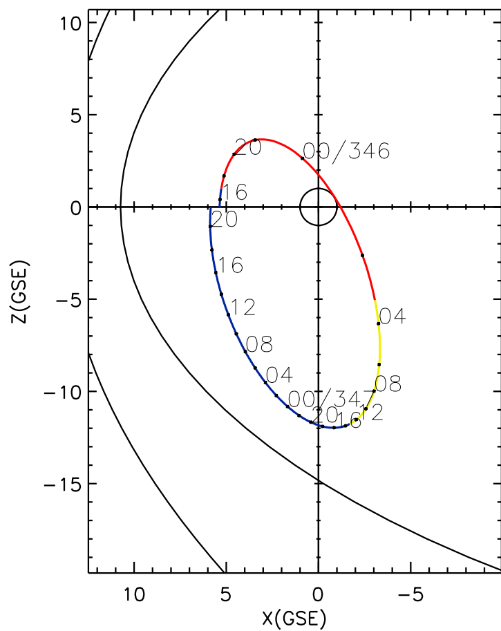
CLUSTER 2 orbit 2013 345 (12/11) 15:21 UT to 2013 347 (12/13) 21:36 UT
