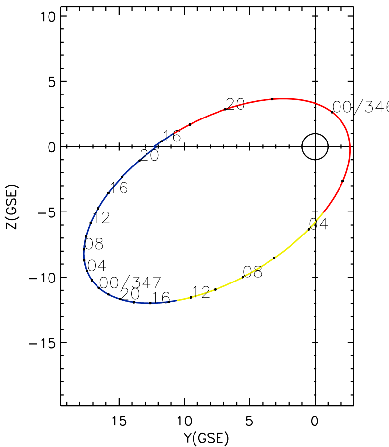
CLUSTER 2 orbit 2013 345 (12/11) 15:21 UT to 2013 347 (12/13) 21:36 UT
