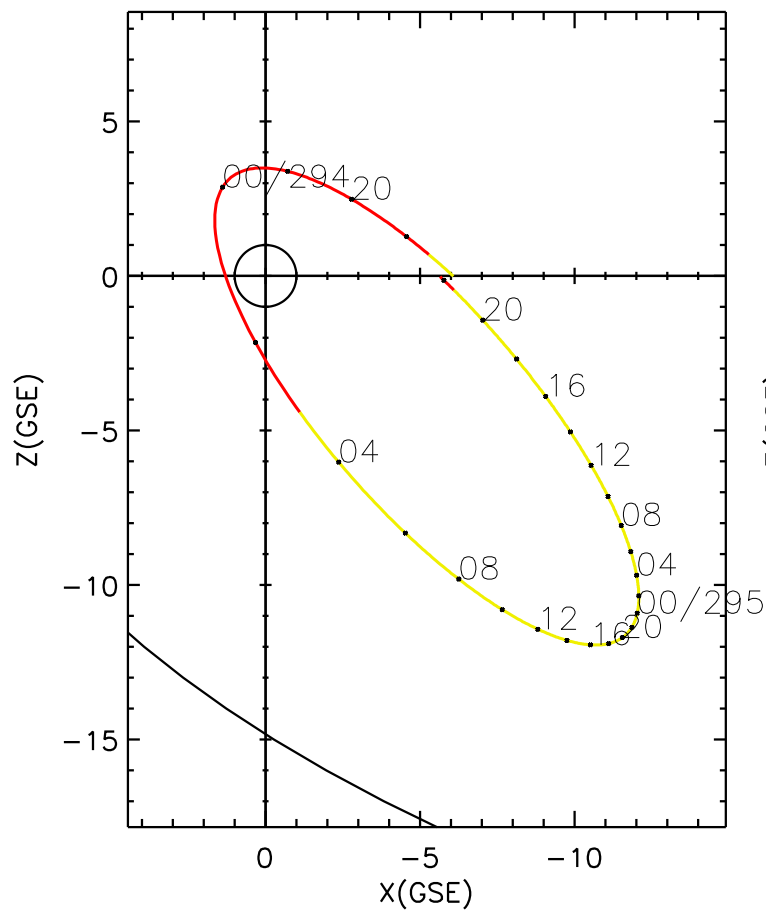
CLUSTER 2 orbit 2013 293 (10/20) 16:01 UT to 2013 295 (10/22) 22:11 UT
