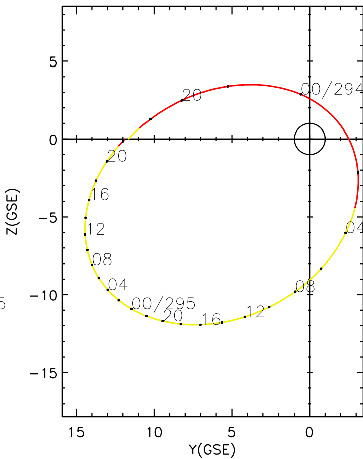
CLUSTER 2 orbit 2013 293 (10/20) 16:01 UT to 2013 295 (10/22) 22:11 UT
