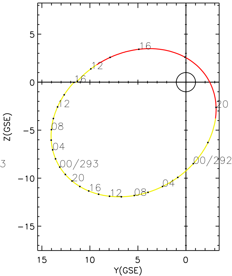
CLUSTER 2 orbit 2013 291 (10/18) 09:46 UT to 2013 293 (10/20) 16:01 UT
