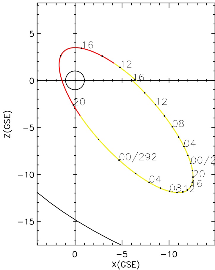
CLUSTER 2 orbit 2013 291 (10/18) 09:46 UT to 2013 293 (10/20) 16:01 UT
