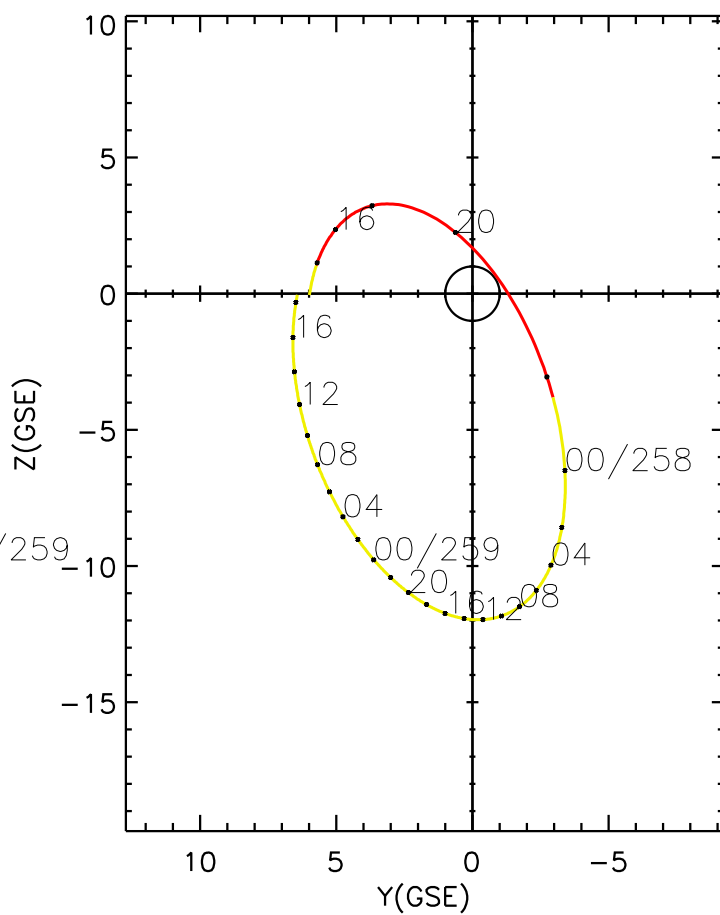
CLUSTER 2 orbit 2013 257 (09/14) 12:11 UT to 2013 259 (09/16) 18:26 UT
