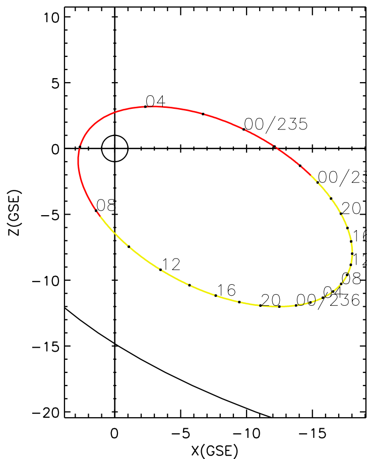
CLUSTER 2 orbit 2013 234 (08/22) 21:41 UT to 2013 237 (08/25) 03:56 UT
