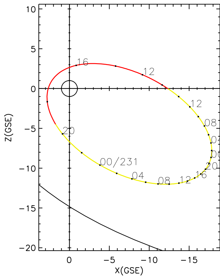
CLUSTER 2 orbit 2013 230 (08/18) 09:16 UT to 2013 232 (08/20) 15:31 UT
