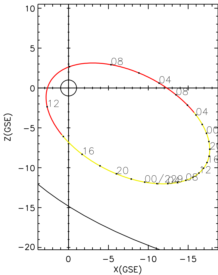
CLUSTER 2 orbit 2013 228 (08/16) 03:01 UT to 2013 230 (08/18) 09:16 UT
