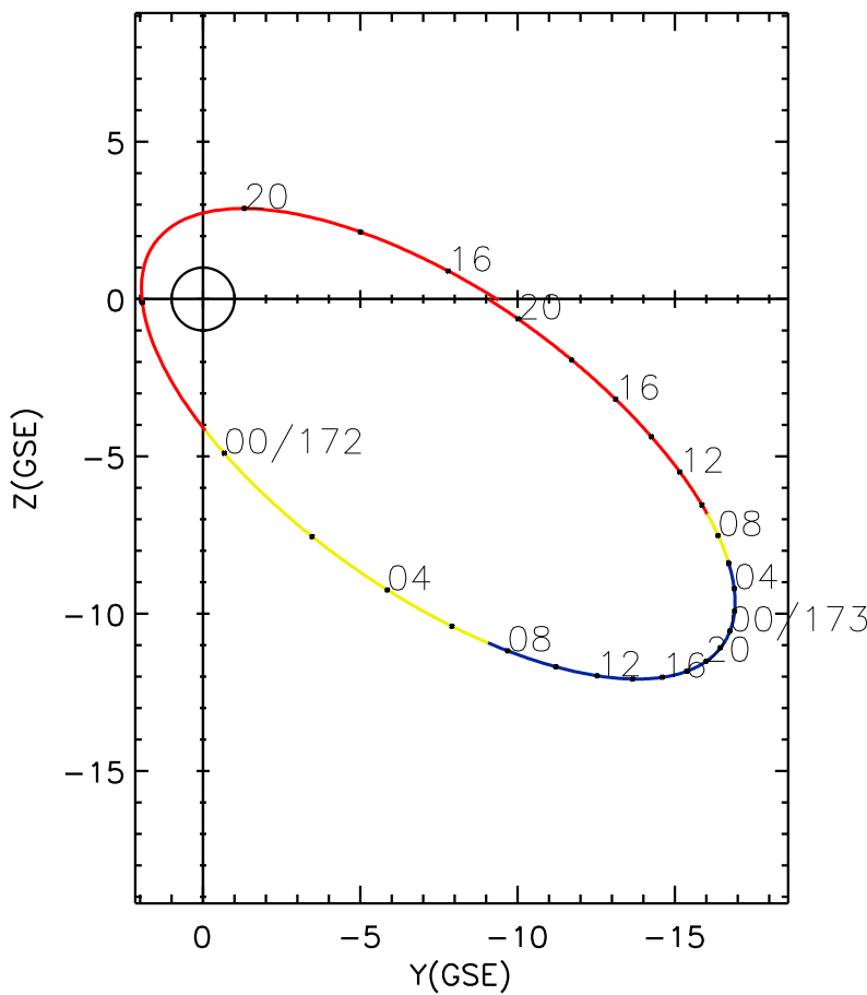
CLUSTER 2 orbit 2013 171 (06/20) 14:36 UT to 2013 173 (06/22) 20:56 UT
