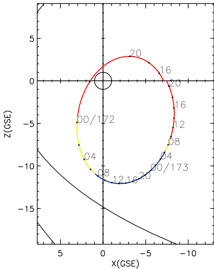
CLUSTER 2 orbit 2013 171 (06/20) 14:36 UT to 2013 173 (06/22) 20:56 UT
