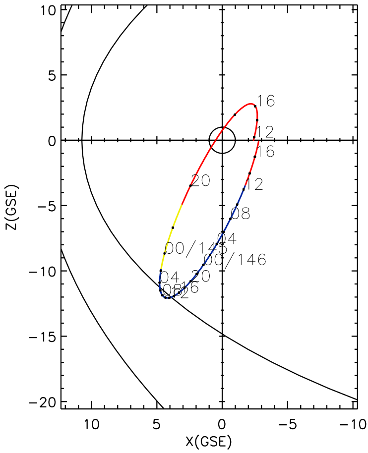
CLUSTER 2 orbit 2013 144 (05/24) 11:36 UT to 2013 146 (05/26) 17:51 UT
