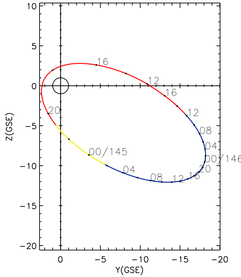
CLUSTER 2 orbit 2013 144 (05/24) 11:36 UT to 2013 146 (05/26) 17:51 UT
