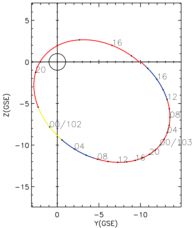
CLUSTER 2 orbit 2013 101 (04/11) 12:51 UT to 2013 103 (04/13) 19:06 UT
