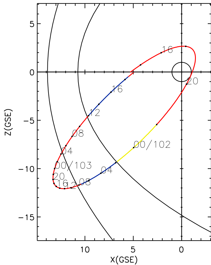
CLUSTER 2 orbit 2013 101 (04/11) 12:51 UT to 2013 103 (04/13) 19:06 UT
