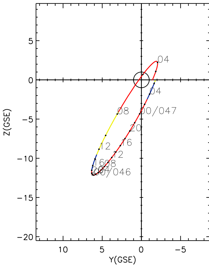
CLUSTER 2 orbit 2013 045 (02/14) 00:21 UT to 2013 047 (02/16) 06:36 UT
