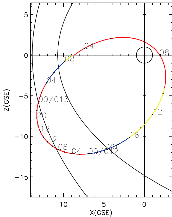
CLUSTER 2 orbit 2013 011 (01/11) 02:46 UT to 2013 013 (01/13) 09:01 UT
