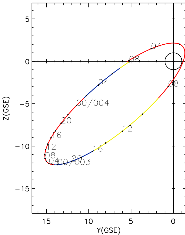
CLUSTER 2 orbit 2013 002 (01/02) 01:46 UT to 2013 004 (01/04) 08:01 UT
