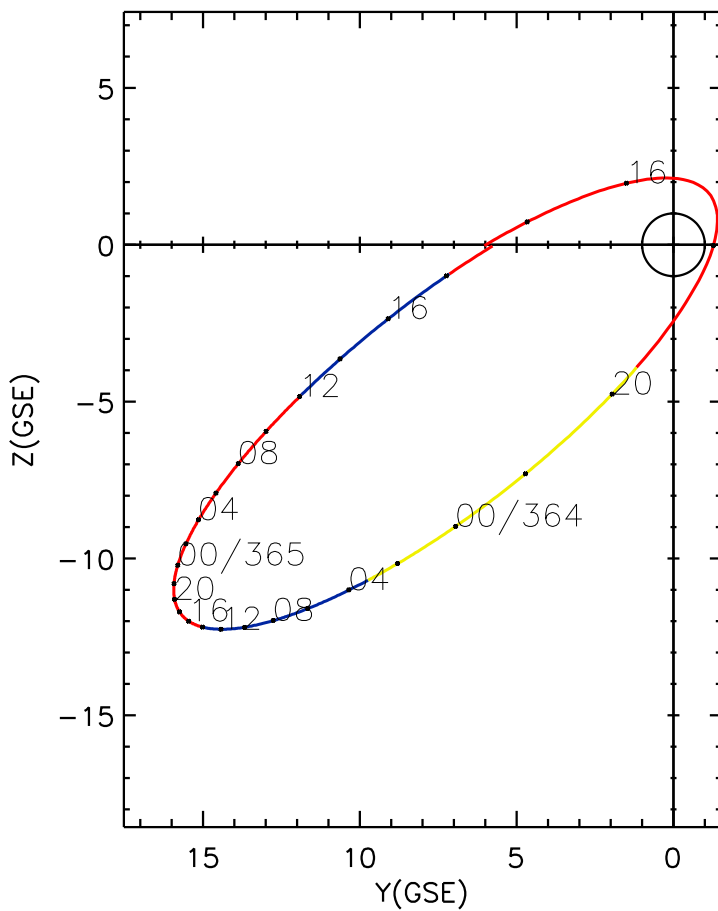
CLUSTER 2 orbit 2012 363 (12/28) 12:56 UT to 2012 365 (12/30) 19:21 UT
