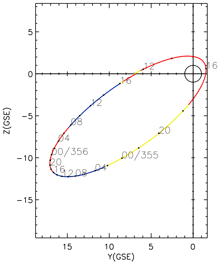
CLUSTER 2 orbit 2012 354 (12/19) 11:11 UT to 2012 356 (12/21) 17:36 UT
