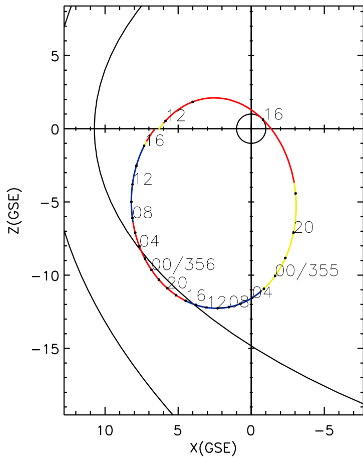
CLUSTER 2 orbit 2012 354 (12/19) 11:11 UT to 2012 356 (12/21) 17:36 UT
