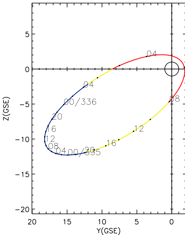
CLUSTER 2 orbit 2012 334 (11/29) 01:16 UT to 2012 336 (12/01) 07:41 UT
