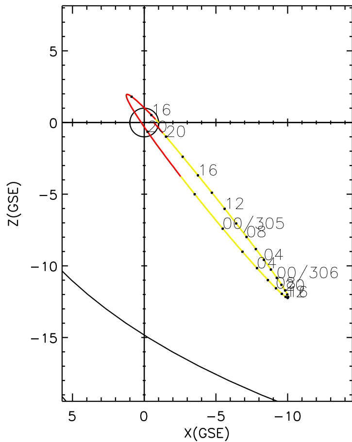
CLUSTER 2 orbit 2012 304 (10/30) 15:16 UT to 2012 306 (11/01) 21:21 UT
