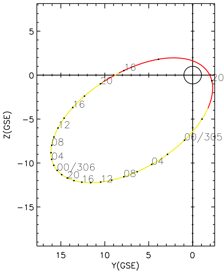
CLUSTER 2 orbit 2012 304 (10/30) 15:16 UT to 2012 306 (11/01) 21:21 UT
