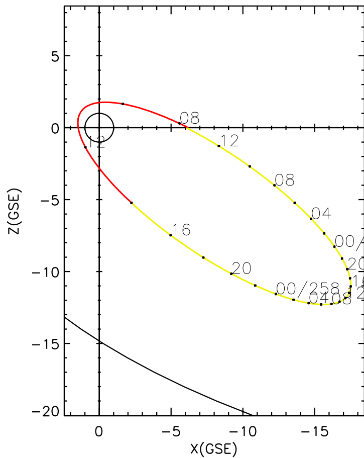
CLUSTER 2 orbit 2012 257 (09/13) 07:36 UT to 2012 259 (09/15) 13:41 UT
