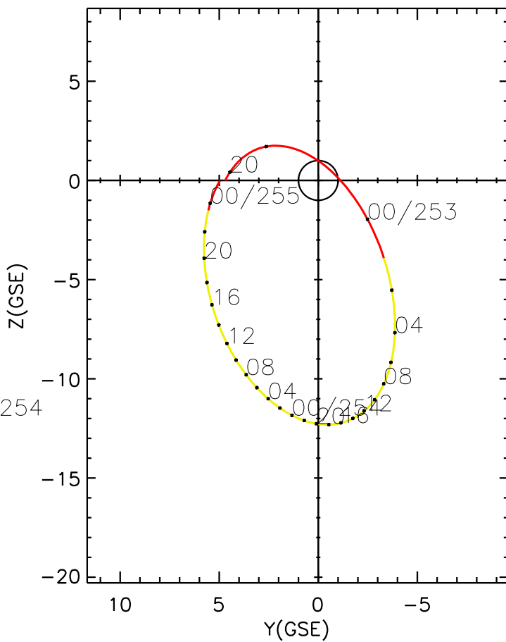
CLUSTER 2 orbit 2012 252 (09/08) 19:26 UT to 2012 255 (09/11) 01:31 UT
