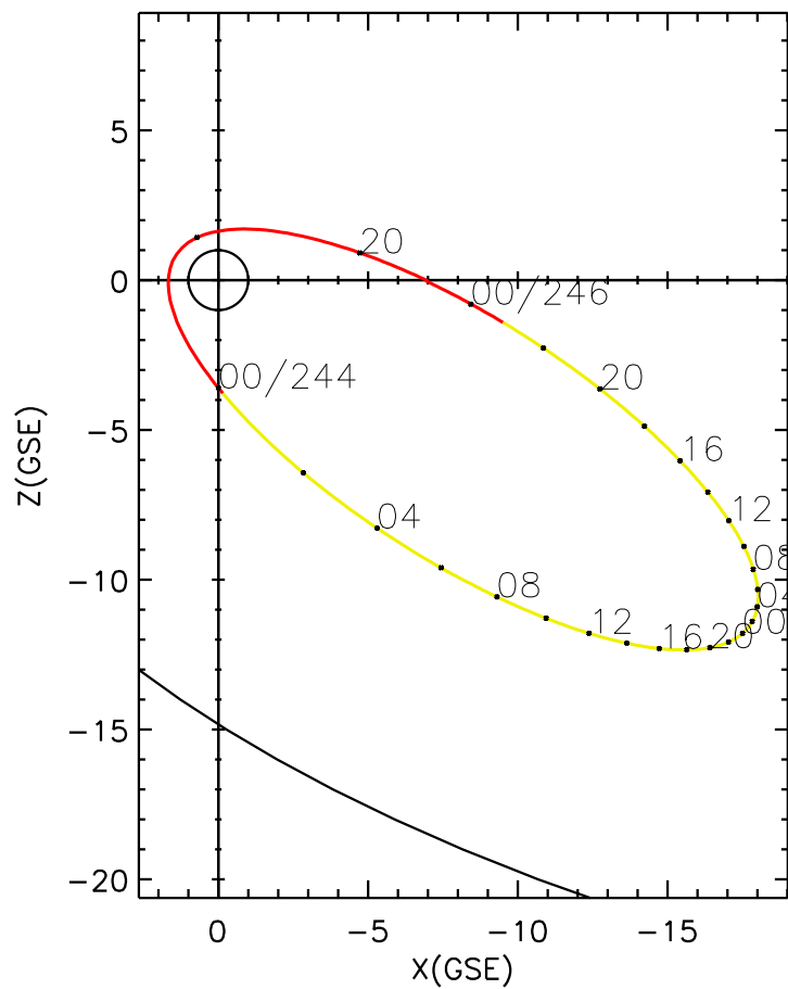
CLUSTER 2 orbit 2012 243 (08/30) 18:46 UT to 2012 246 (09/02) 01:01 UT
