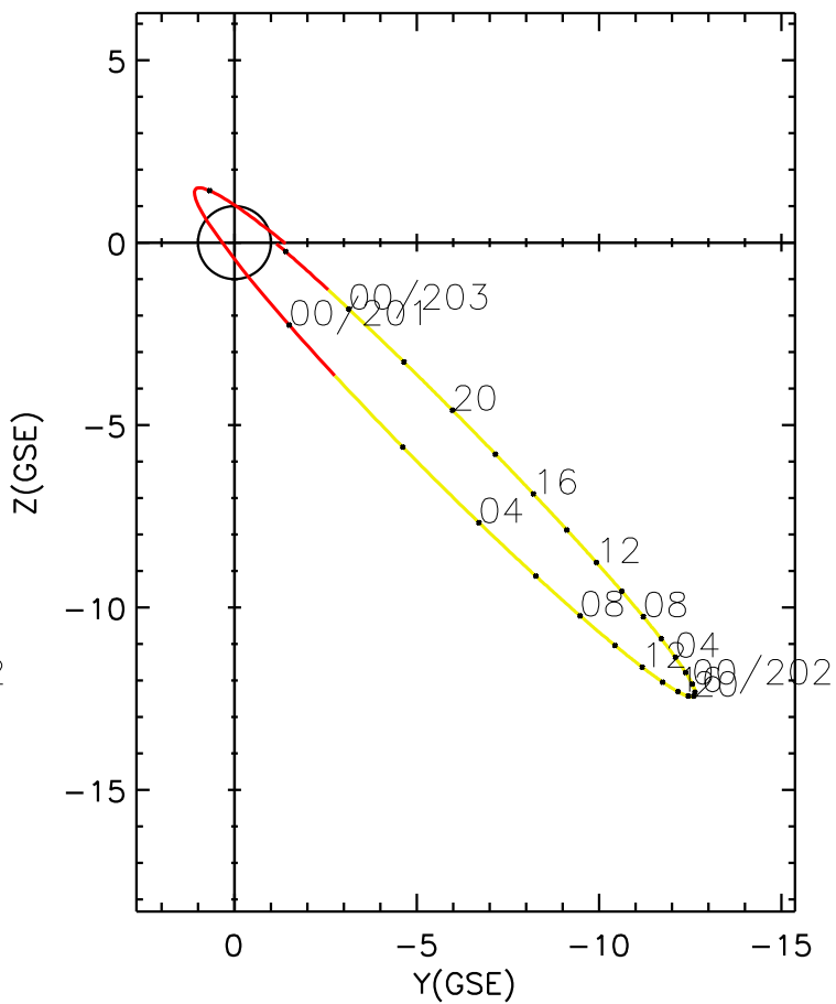
CLUSTER 2 orbit 2012 200 (07/18) 20:01 UT to 2012 203 (07/21) 02:16 UT
