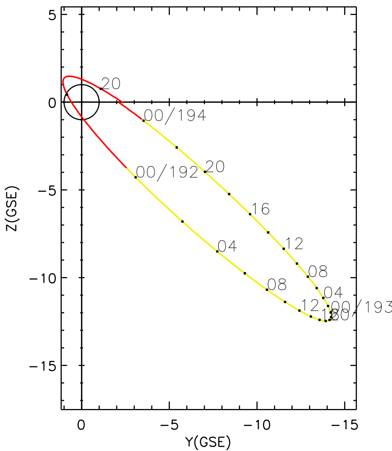
CLUSTER 2 orbit 2012 191 (07/09) 19:01 UT to 2012 194 (07/12) 01:16 UT
