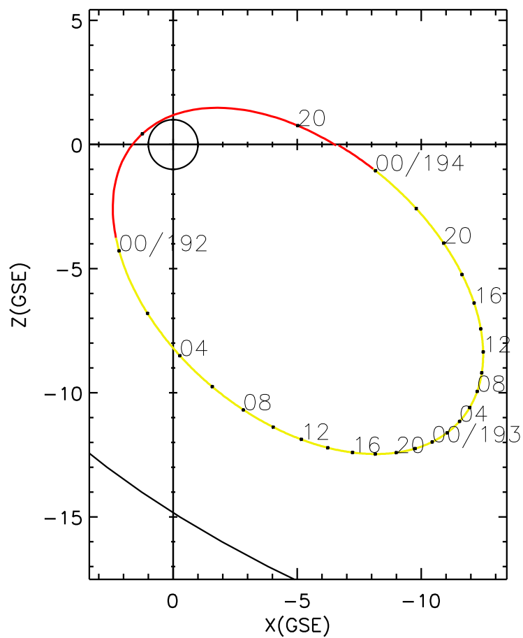
CLUSTER 2 orbit 2012 191 (07/09) 19:01 UT to 2012 194 (07/12) 01:16 UT
