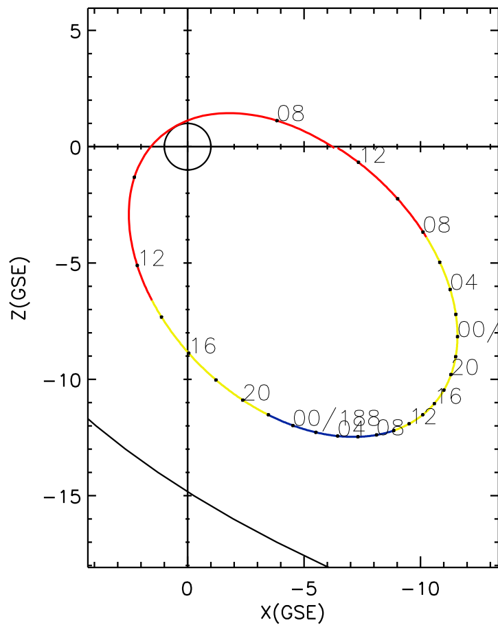
CLUSTER 2 orbit 2012 187 (07/05) 06:31 UT to 2012 189 (07/07) 12:46 UT
