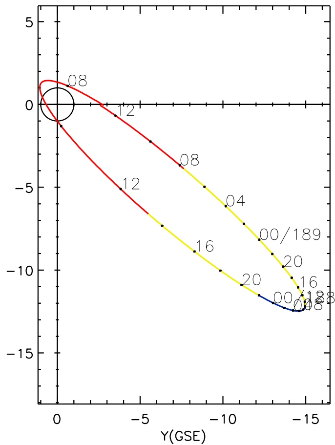
CLUSTER 2 orbit 2012 187 (07/05) 06:31 UT to 2012 189 (07/07) 12:46 UT
