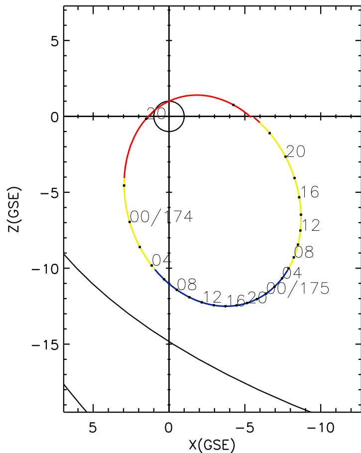
CLUSTER 2 orbit 2012 173 (06/21) 17:01 UT to 2012 175 (06/23) 23:16 UT
