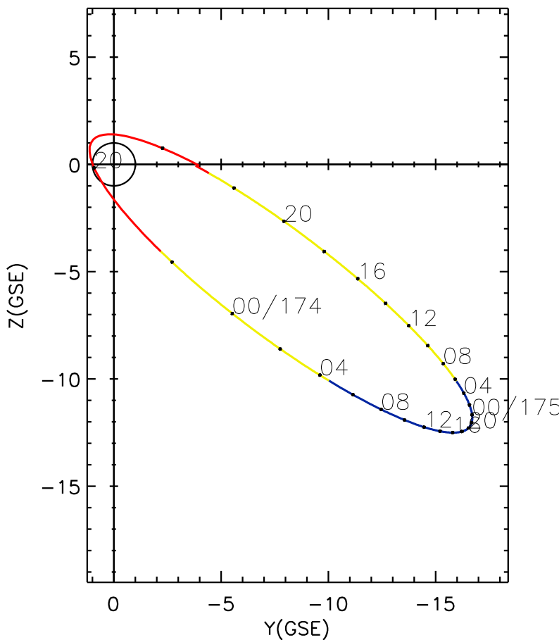
CLUSTER 2 orbit 2012 173 (06/21) 17:01 UT to 2012 175 (06/23) 23:16 UT
