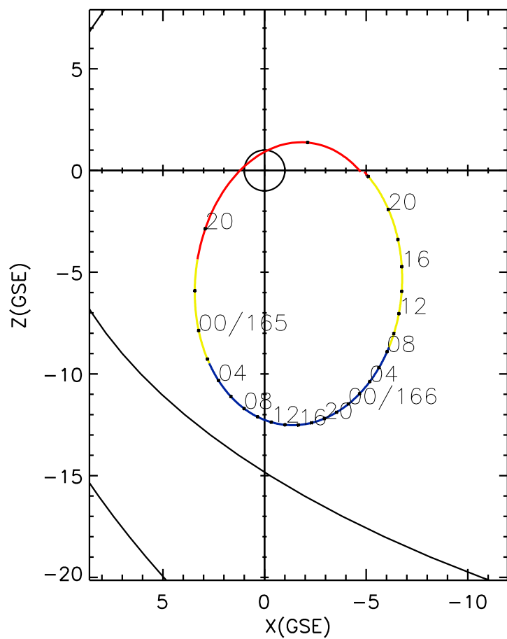
CLUSTER 2 orbit 2012 164 (06/12) 16:01 UT to 2012 166 (06/14) 22:16 UT
