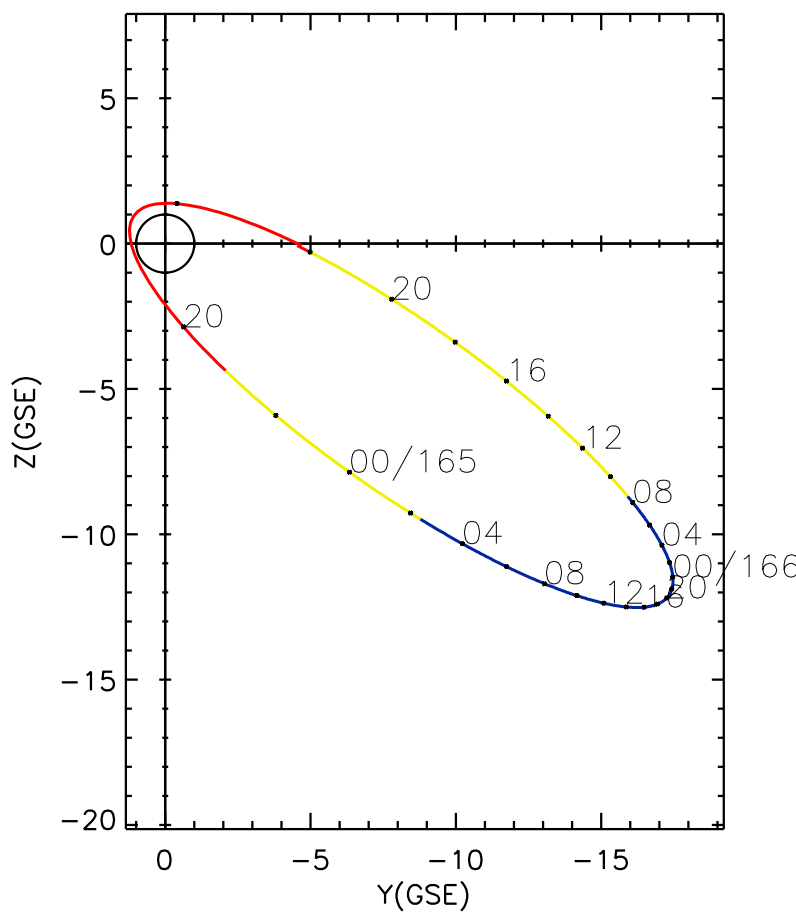
CLUSTER 2 orbit 2012 164 (06/12) 16:01 UT to 2012 166 (06/14) 22:16 UT
