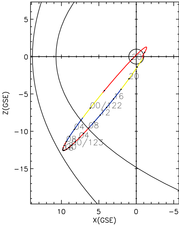
CLUSTER 2 orbit 2012 121 (04/30) 17:21 UT to 2012 123 (05/02) 23:36 UT
