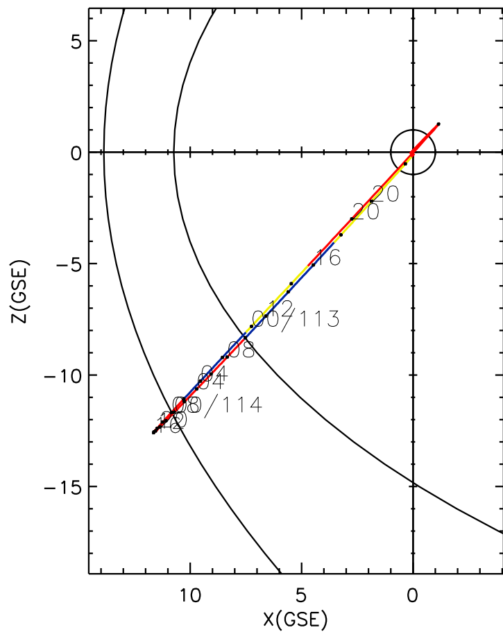
CLUSTER 2 orbit 2012 112 (04/21) 16:16 UT to 2012 114 (04/23) 22:31 UT
