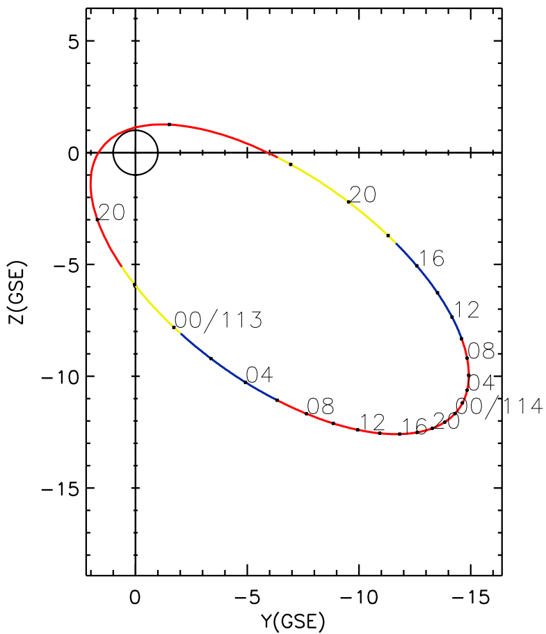
CLUSTER 2 orbit 2012 112 (04/21) 16:16 UT to 2012 114 (04/23) 22:31 UT
