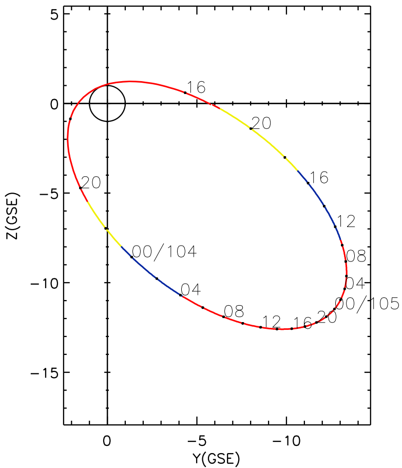
CLUSTER 2 orbit 2012 103 (04/12) 15:16 UT to 2012 105 (04/14) 21:31 UT
