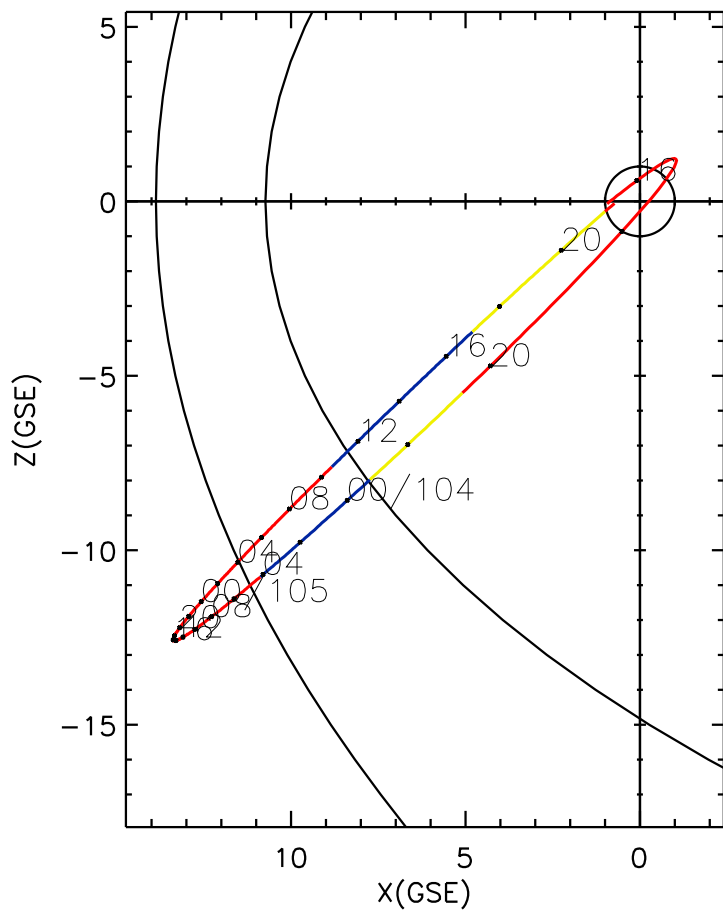
CLUSTER 2 orbit 2012 103 (04/12) 15:16 UT to 2012 105 (04/14) 21:31 UT
