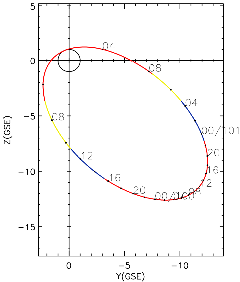
CLUSTER 2 orbit 2012 099 (04/08) 02:46 UT to 2012 101 (04/10) 09:01 UT
