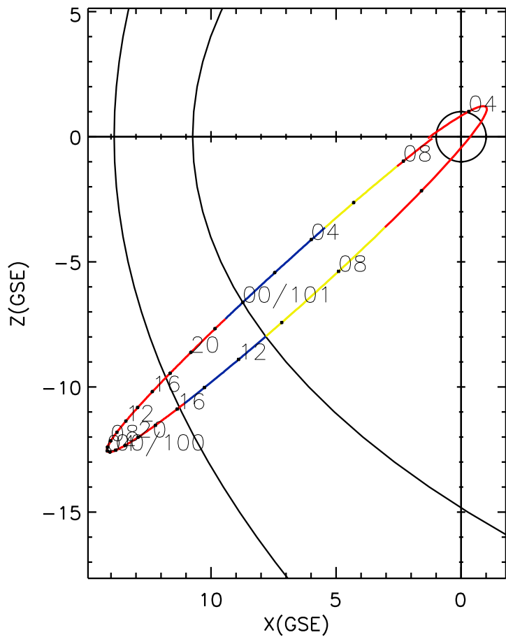
CLUSTER 2 orbit 2012 099 (04/08) 02:46 UT to 2012 101 (04/10) 09:01 UT
