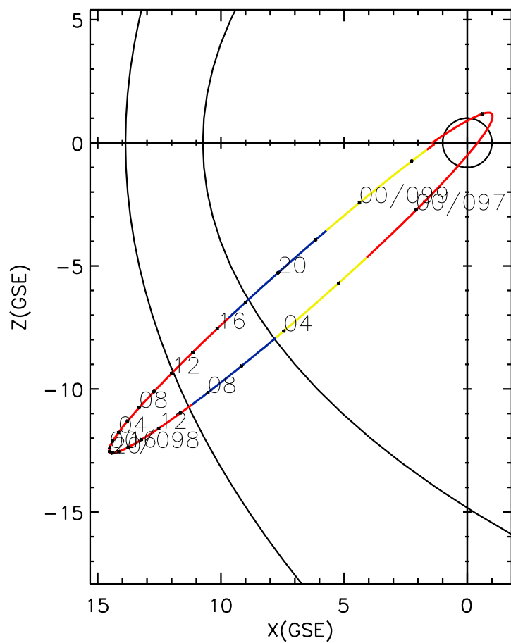
CLUSTER 2 orbit 2012 096 (04/05) 20:31 UT to 2012 099 (04/08) 02:46 UT
