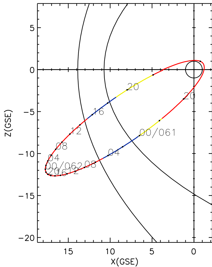
CLUSTER 2 orbit 2012 060 (02/29) 16:21 UT to 2012 062 (03/02) 22:36 UT
