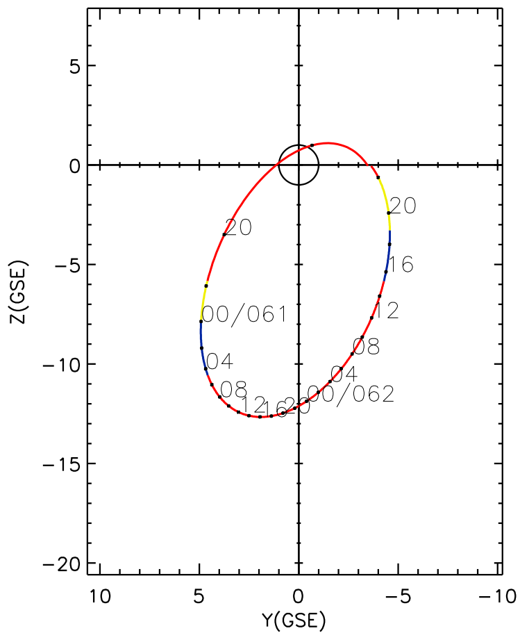
CLUSTER 2 orbit 2012 060 (02/29) 16:21 UT to 2012 062 (03/02) 22:36 UT
