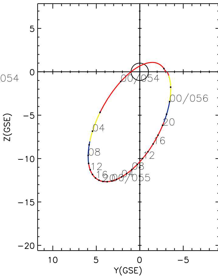
CLUSTER 2 orbit 2012 053 (02/22) 21:36 UT to 2012 056 (02/25) 03:51 UT
