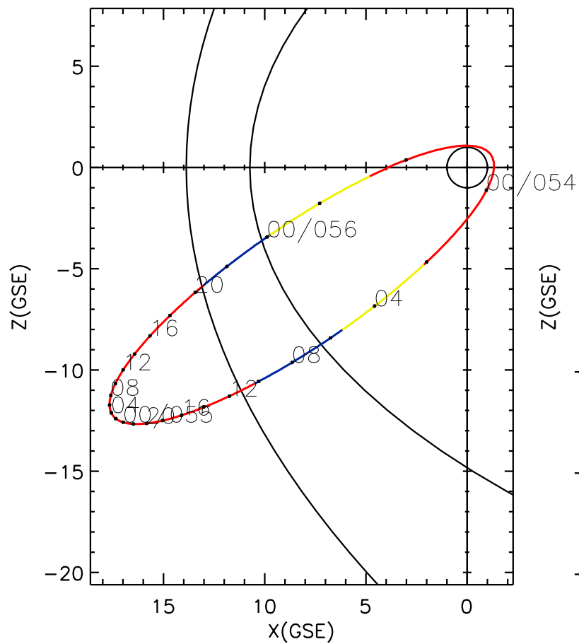
CLUSTER 2 orbit 2012 053 (02/22) 21:36 UT to 2012 056 (02/25) 03:51 UT
