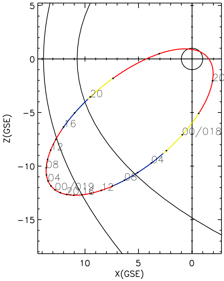
CLUSTER 2 orbit 2012 017 (01/17) 17:31 UT to 2012 019 (01/19) 23:46 UT
