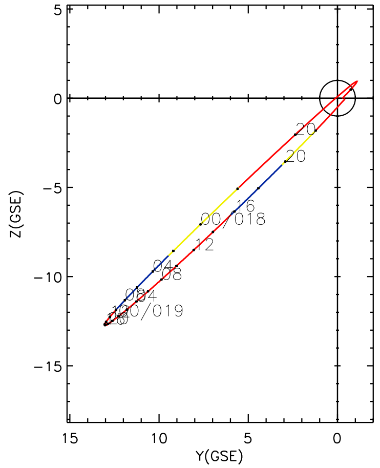
CLUSTER 2 orbit 2012 017 (01/17) 17:31 UT to 2012 019 (01/19) 23:46 UT
