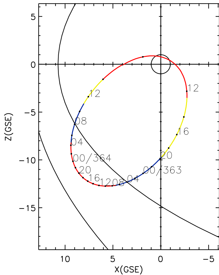
CLUSTER 2 orbit 2011 362 (12/28) 09:11 UT to 2011 364 (12/30) 15:26 UT
