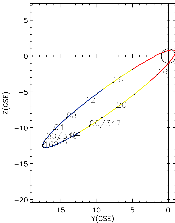
CLUSTER 2 orbit 2011 346 (12/12) 13:26 UT to 2011 348 (12/14) 19:41 UT
