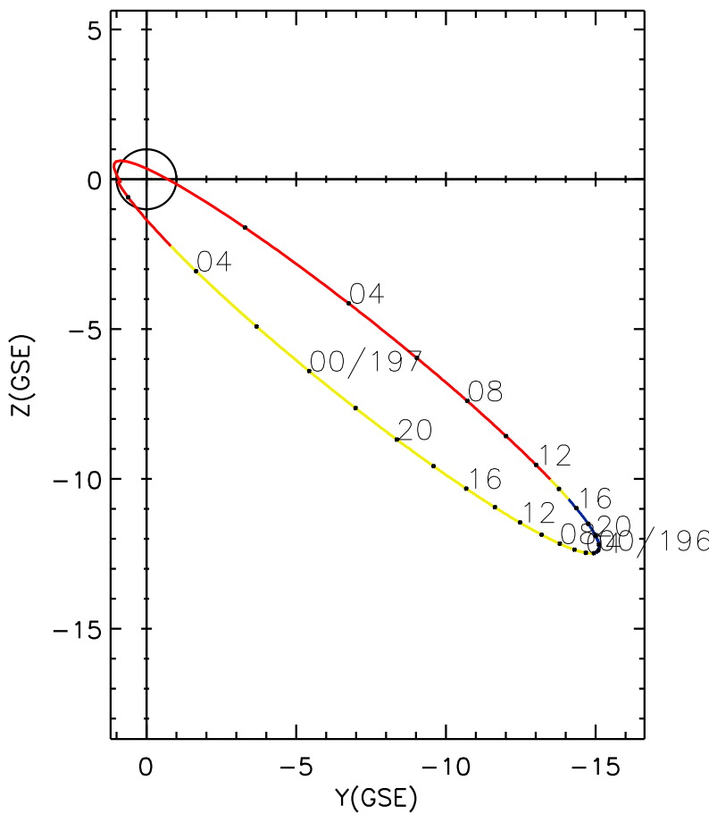
CLUSTER 2 orbit 2011 195 (07/14) 00:06 UT to 2011 197 (07/16) 06:21 UT
