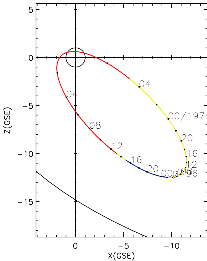
CLUSTER 2 orbit 2011 195 (07/14) 00:06 UT to 2011 197 (07/16) 06:21 UT
