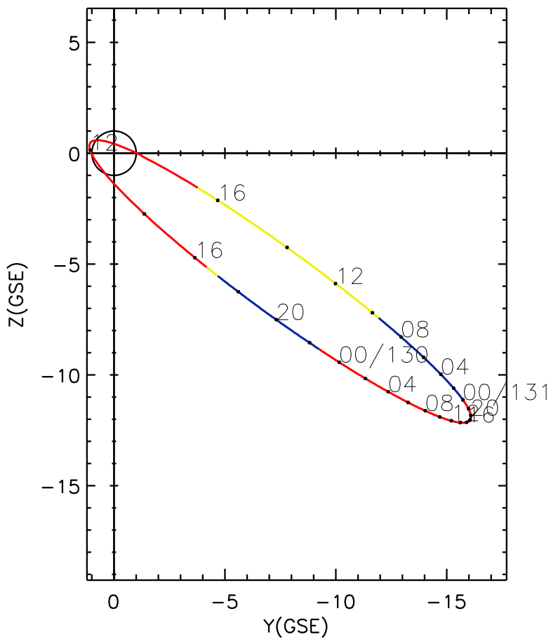
CLUSTER 2 orbit 2011 129 (05/09) 11:06 UT to 2011 131 (05/11) 17:21 UT
