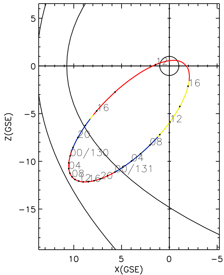
CLUSTER 2 orbit 2011 129 (05/09) 11:06 UT to 2011 131 (05/11) 17:21 UT
