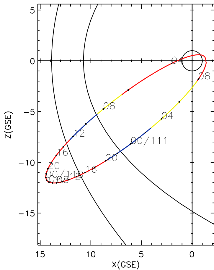
CLUSTER 2 orbit 2011 109 (04/19) 02:51 UT to 2011 111 (04/21) 09:06 UT
