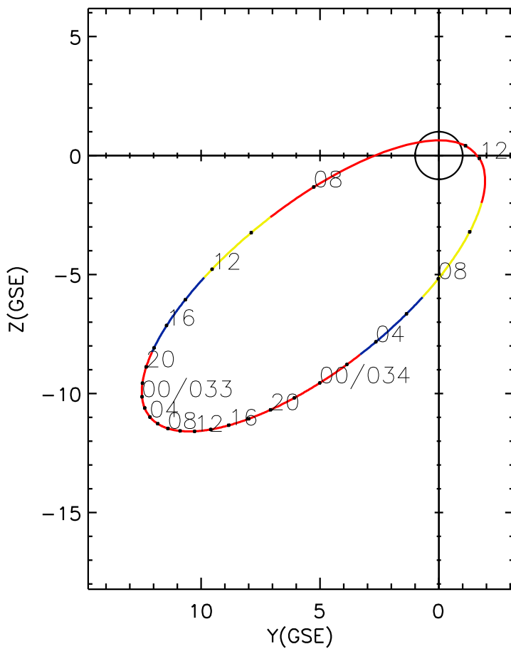
CLUSTER 2 orbit 2011 032 (02/01) 05:46 UT to 2011 034 (02/03) 12:01 UT
