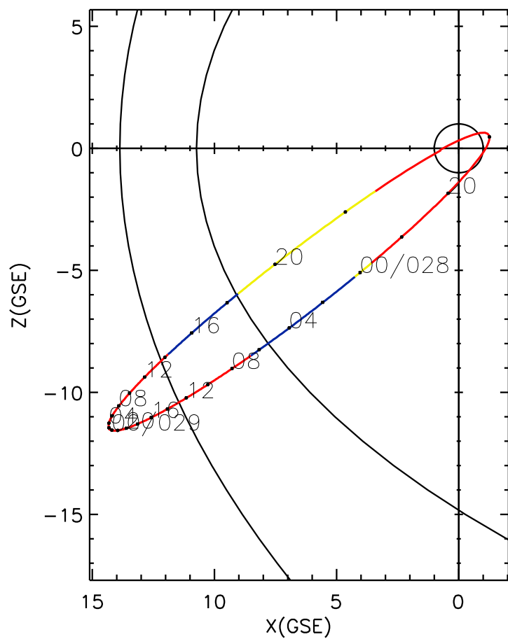
CLUSTER 2 orbit 2011 027 (01/27) 17:16 UT to 2011 029 (01/29) 23:31 UT
