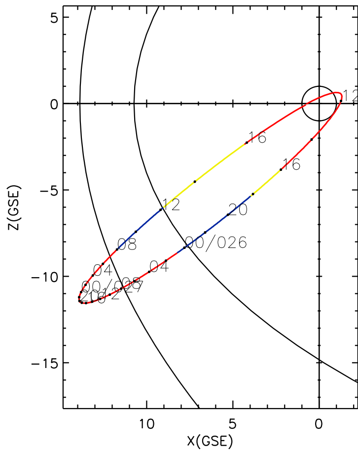
CLUSTER 2 orbit 2011 025 (01/25) 11:01 UT to 2011 027 (01/27) 17:16 UT
