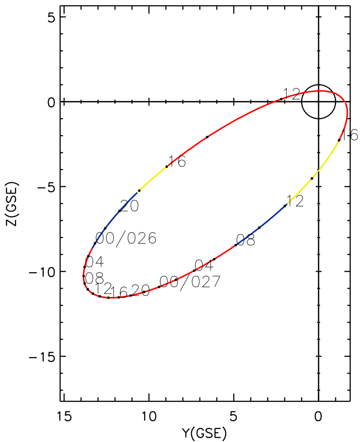
CLUSTER 2 orbit 2011 025 (01/25) 11:01 UT to 2011 027 (01/27) 17:16 UT
