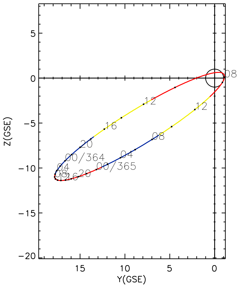
CLUSTER 2 orbit 2010 363 (12/29) 07:56 UT to 2010 365 (12/31) 14:11 UT
