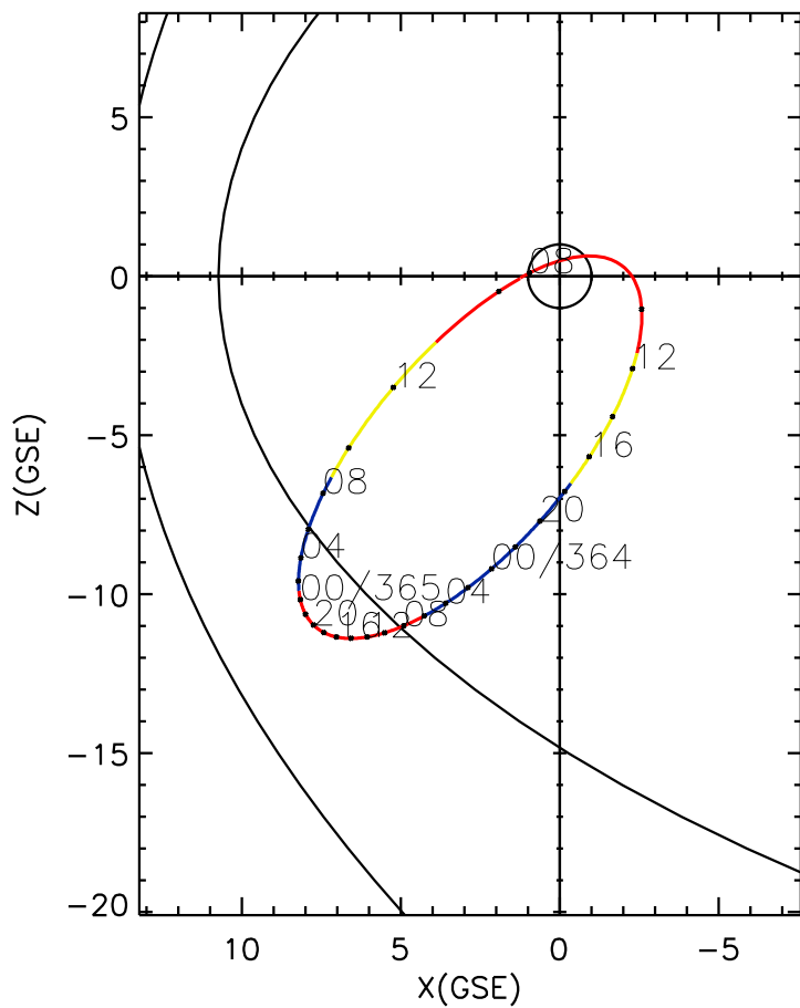
CLUSTER 2 orbit 2010 363 (12/29) 07:56 UT to 2010 365 (12/31) 14:11 UT
