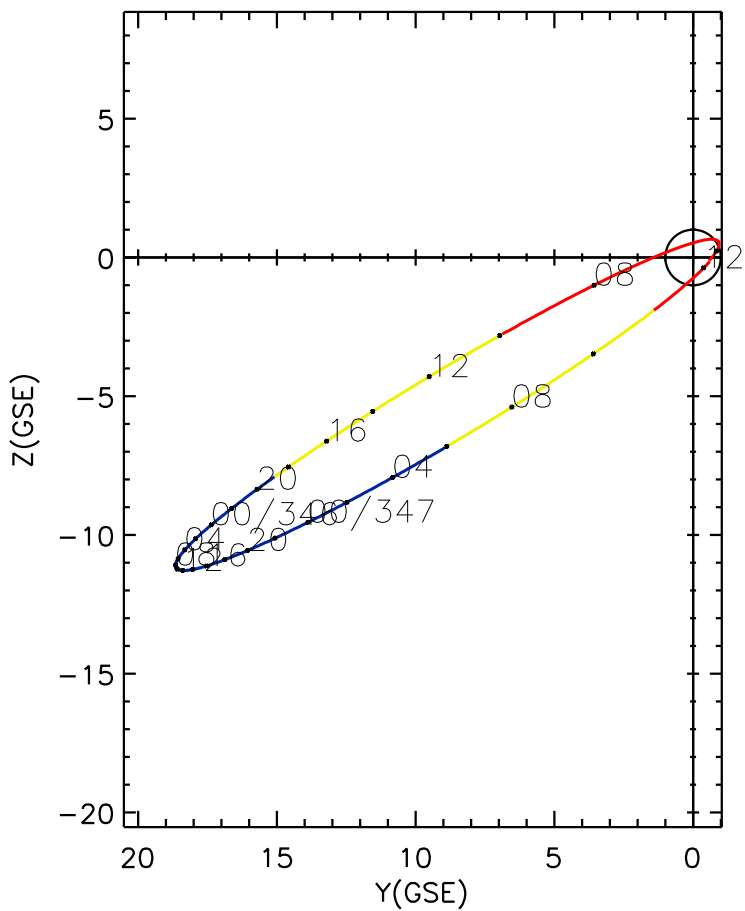
CLUSTER 2 orbit 2010 345 (12/11) 05:51 UT to 2010 347 (12/13) 12:06 UT
