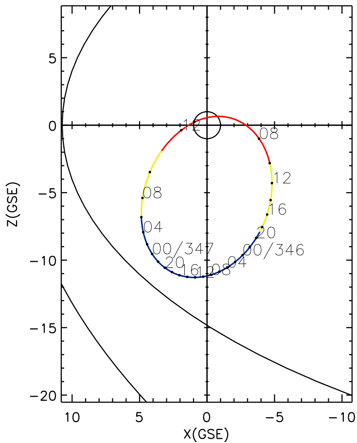
CLUSTER 2 orbit 2010 345 (12/11) 05:51 UT to 2010 347 (12/13) 12:06 UT
