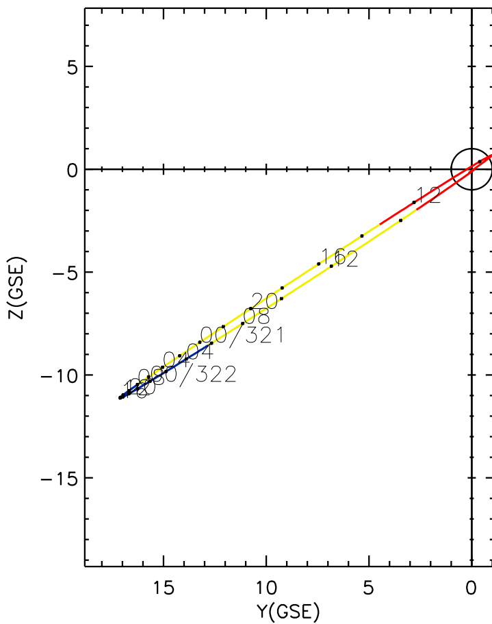
CLUSTER 2 orbit 2010 320 (11/16) 09:01 UT to 2010 322 (11/18) 15:21 UT
